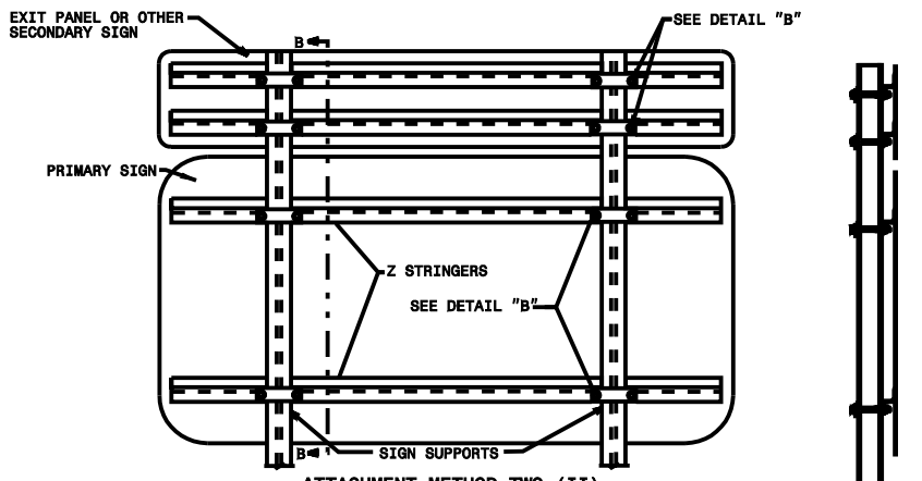
ATTACHMENT METHOD TWO (II) (EXIT PANEL OR OTHER SECONDARY SIGN ATTACHED TO PRIMARY SIGN SUPPORTS)
