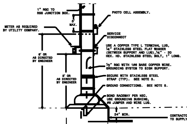
VIEW B-B
