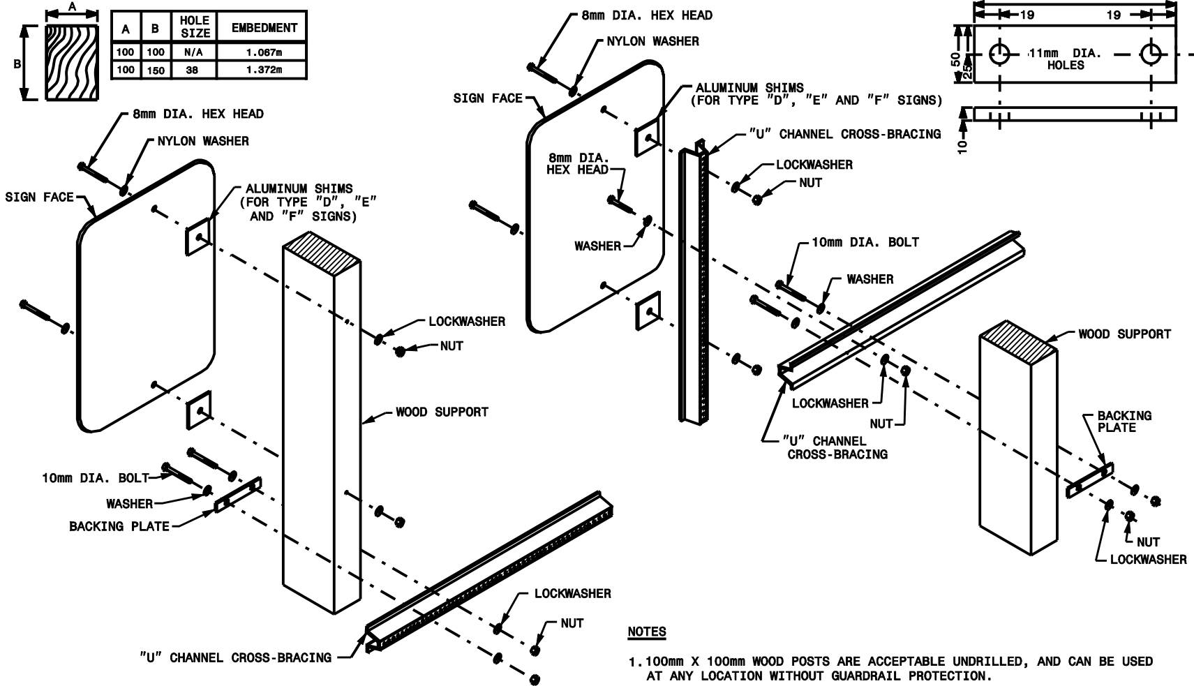
POST SIZE AND DRILLED HOLE SIZE
