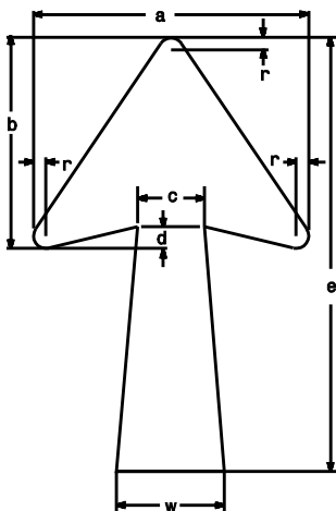
DETAIL OF INTERSTATE ARROW
