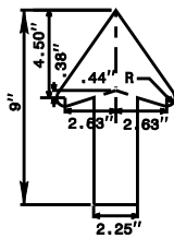
DETAIL OF 6" ARROW
