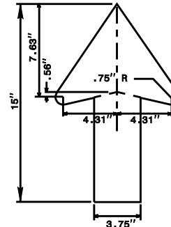
DETAIL OF 10" ARROW
