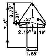
DETAIL OF 5" ARROW
