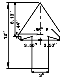
DETAIL OF 8" ARROW
