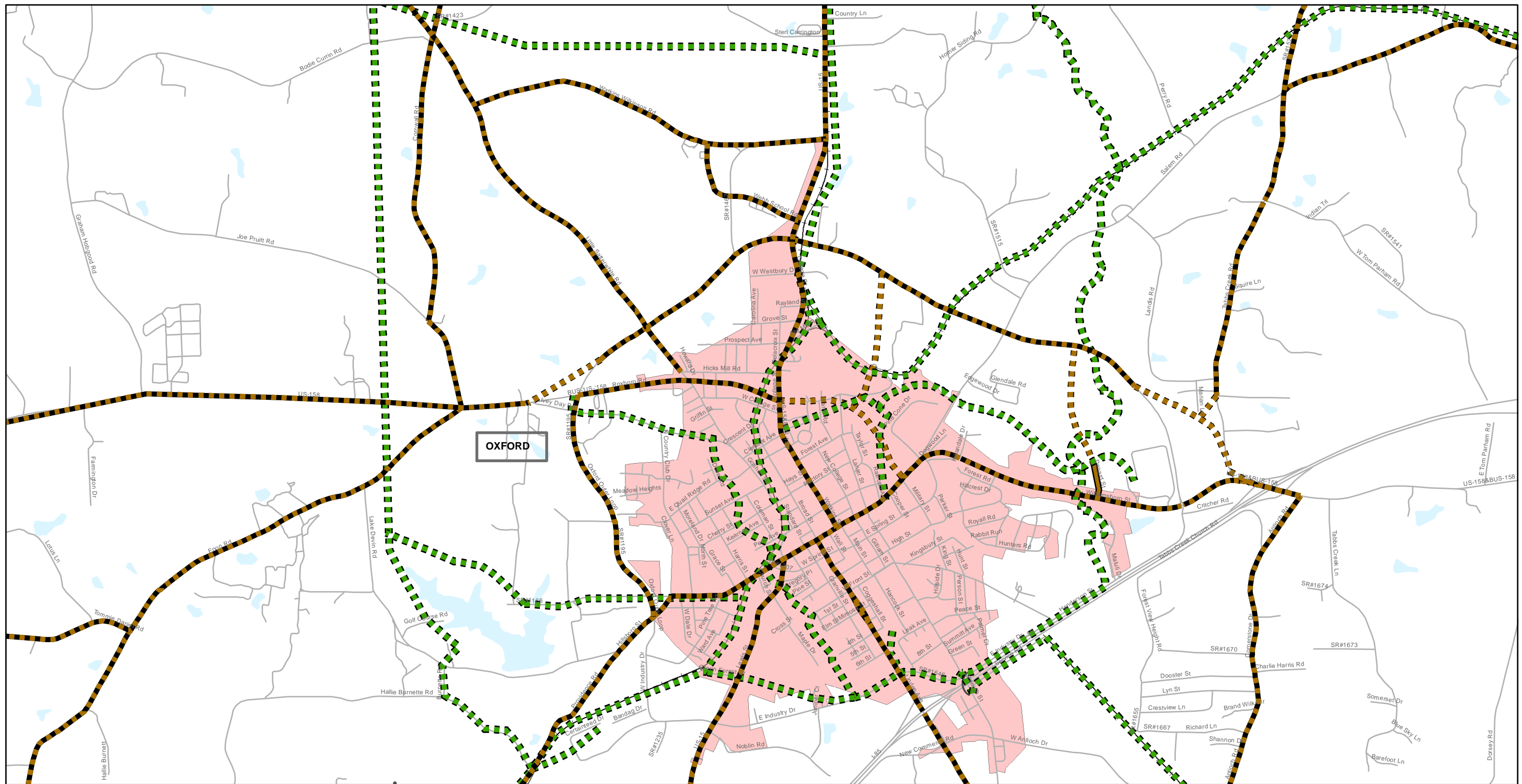
Bicycle Map Granville County Comprehensive Transportation Plan Figure 2 - Sheet 3A of 5 (Oxford) North Carolina
