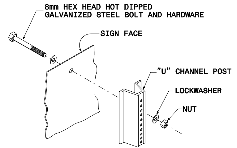
ASSEMBLY DETAIL
