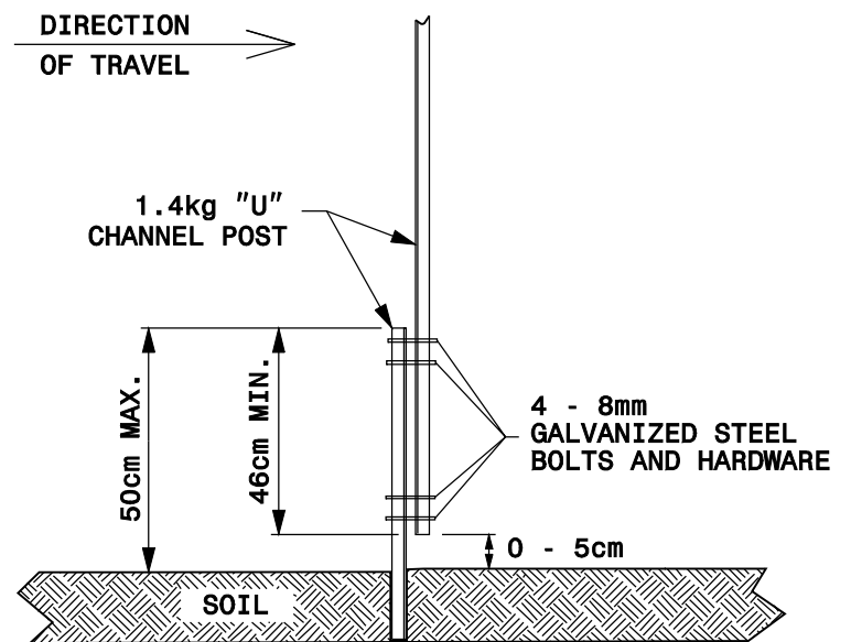
DETAIL FOR SPLICING STEEL U-CHANNEL POST ON SMALL SIGN SUPPORT
