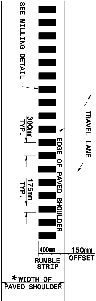
PLAN VIEW PAVED SHOULDER
