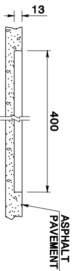
SECTION B-B
