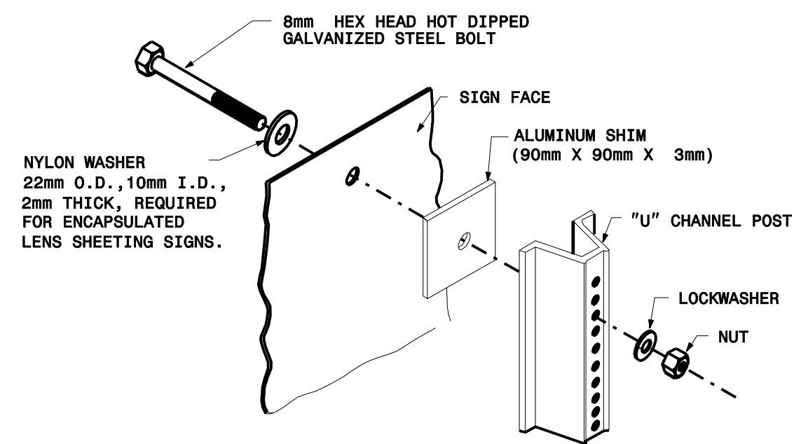
ASSEMBLY DETAIL
