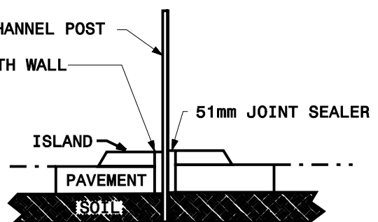
DETAIL FOR INSTALLATION OF CHANNEL POST IN CONCRETE
