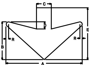
DETAIL OF TYPE "C" ARROW
